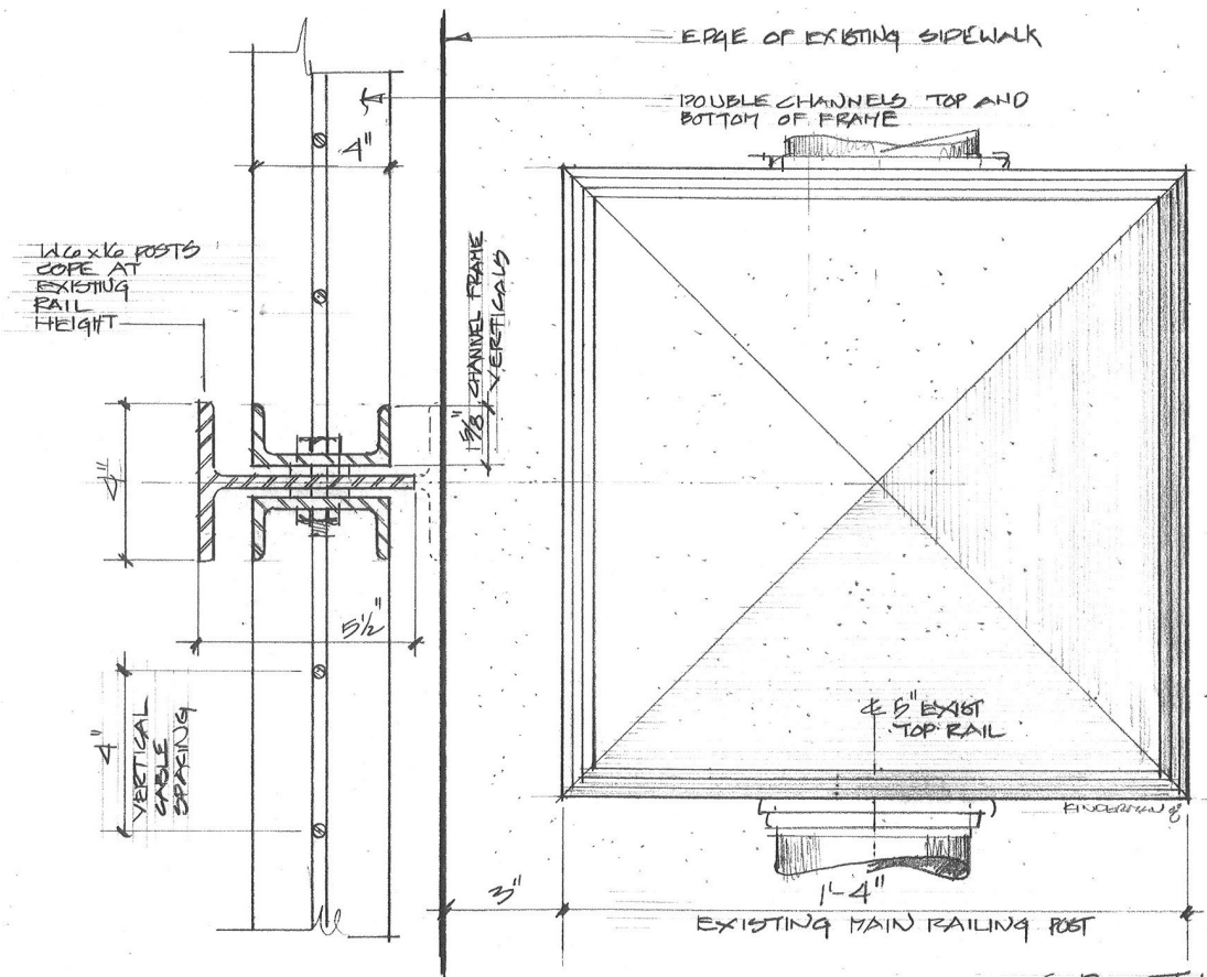
SECTION B-B SHOWING POST AND FRAME CONNECTION
