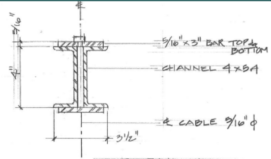
DETAIL A SHOWING TOP & BOTTOM CABLE FRAME
